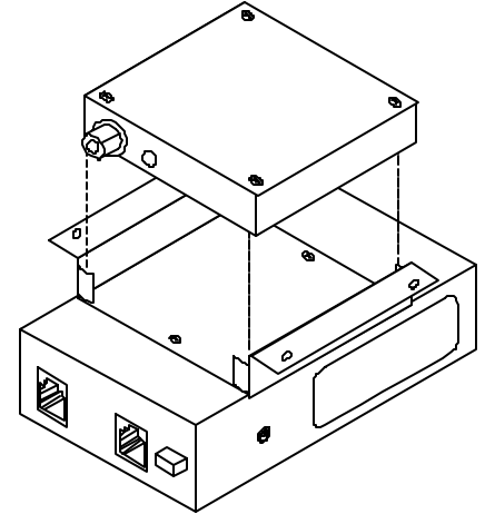
Figure 14: Inserting the CRM into the Bracket
